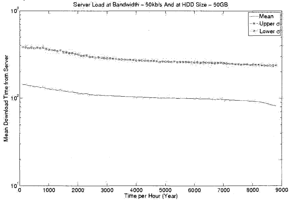
Figure 229: Server Load for H4 case scenario at hard drive size of 50GB and download bandwidth of 50kb/s
