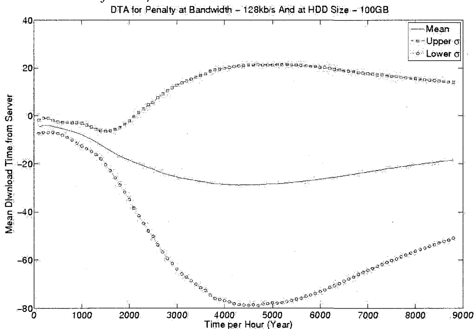
Figure 771: DTA of a difference between H2 and H1 at hard drive size of 100GB and download bandwidth of 128kb/s
