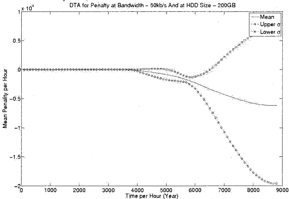
Figure 853: DTA of a difference between H4 and H3 at hard drive size of 200GB and download bandwidth of 50kb/s
