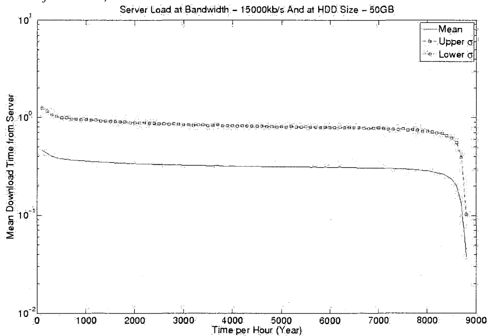
Figure 221: Server Load for H3 case scenario at hard drive size of 50GB and download bandwidth of 15000kb/s
