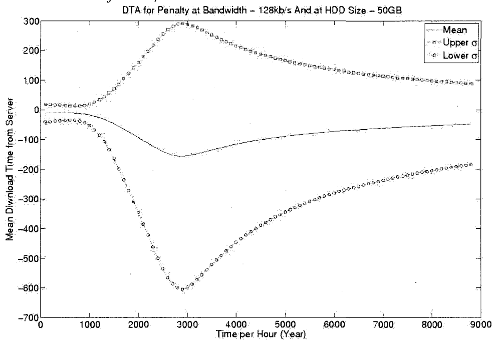
Figure 770: DTA of a difference between H2 and H1 at hard drive size of 50GB and download bandwidth of 128kb/s
