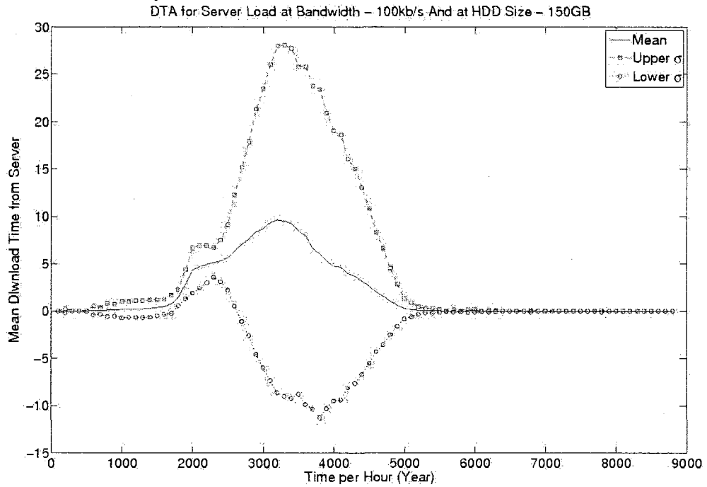
Figure 680: DTA of a difference between H3 and H2 at hard drive size of 150GB and download bandwidth of 100kb/s
