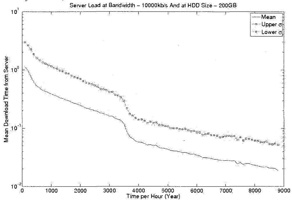
Figure 220: Server Load for H3 case scenario at hard drive size of 200GB and download bandwidth of 10000kb/s
