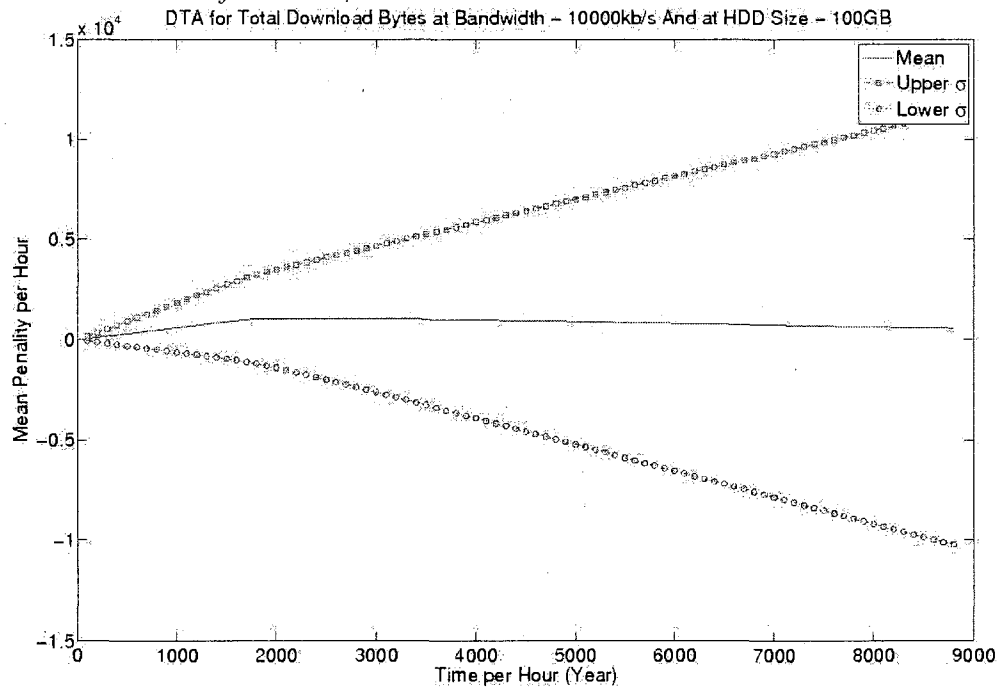
Figure 927: DTA of a difference between H2 and H1 at hard drive size of 100GB and download bandwidth of 10000kb/s
