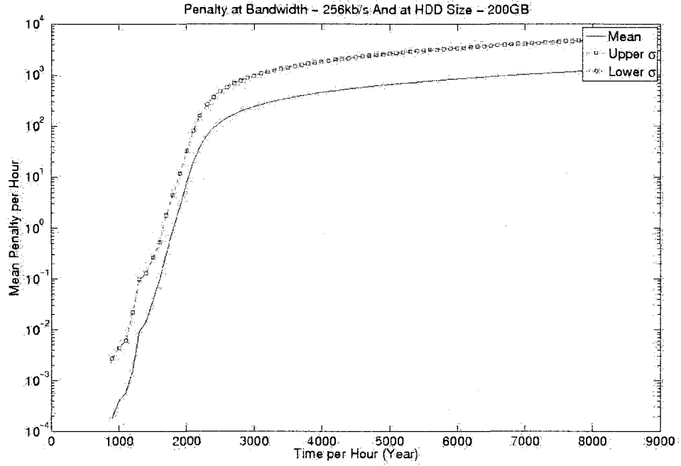
Figure 332: Penalty for H2 case scenario at hard drive size of 200GB and download bandwidth of 256kb/s
