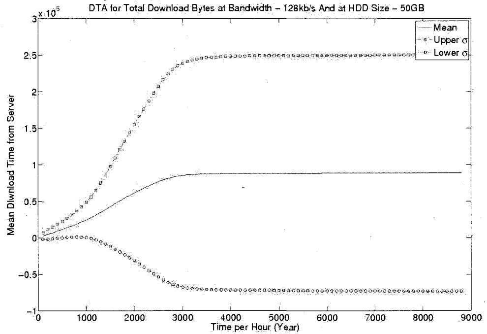
Figure 902: DTA of a difference between H2 and H1 at hard drive size of 50GB and download bandwidth of 128kb/s
